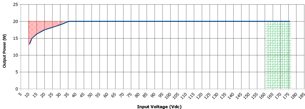
Output Power Derating vs input voltage
