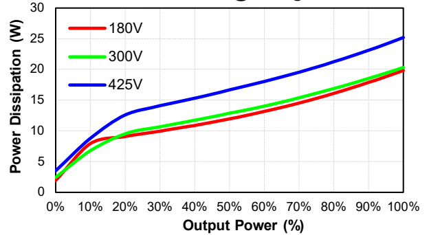
CQB150-300S28-CMFC Pd Vs Po @25 Deg. C
