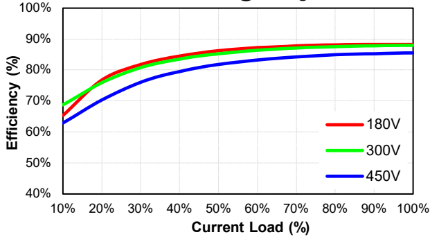
CQB150-300S28-CMFC Eff Vs Io @25 Deg. C
