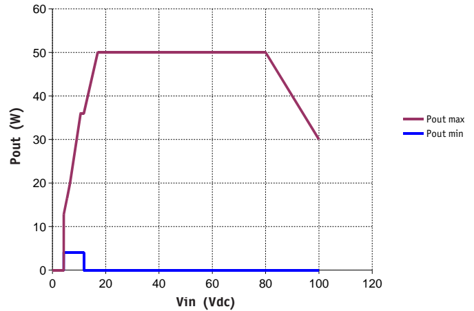
Figure 6 : PGDS-50-0-K Output Power versus Input Voltage
