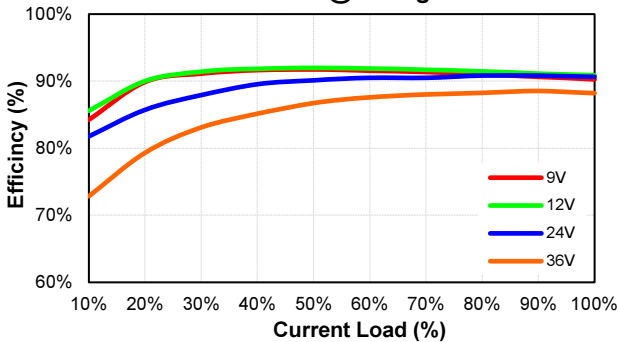
CQB150W-24S28 Eff Vs Io @25 Deg. C
