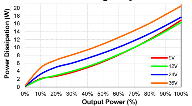
CQB150W-24S28 Pd Vs Po @25 Deg. C
