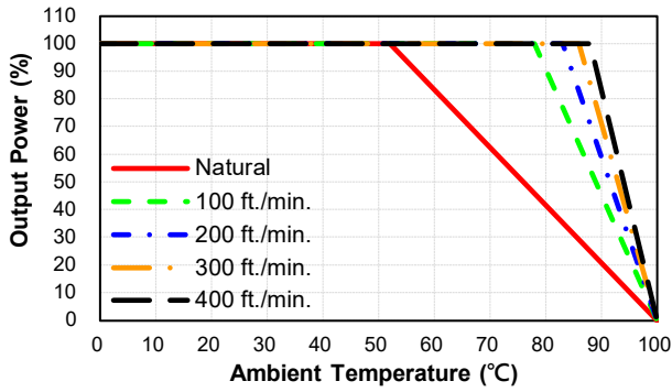
CHB150-110S05/12 Derating Curve with Heatsink HBL210 (Vin=110V)
