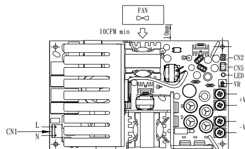
FAN location for CFM351M050 only
